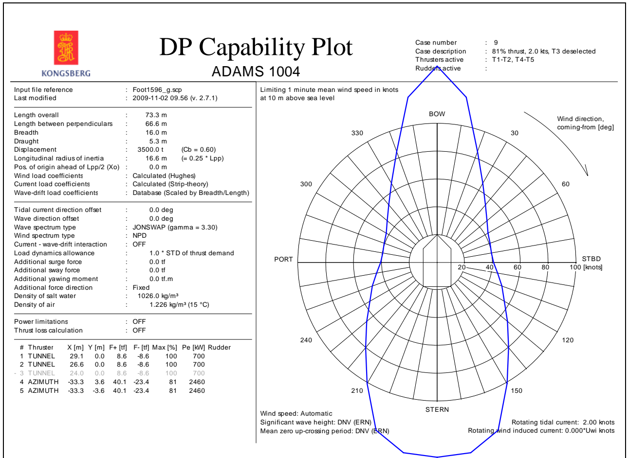
Figure 18: DP capability envelope for case 9.
