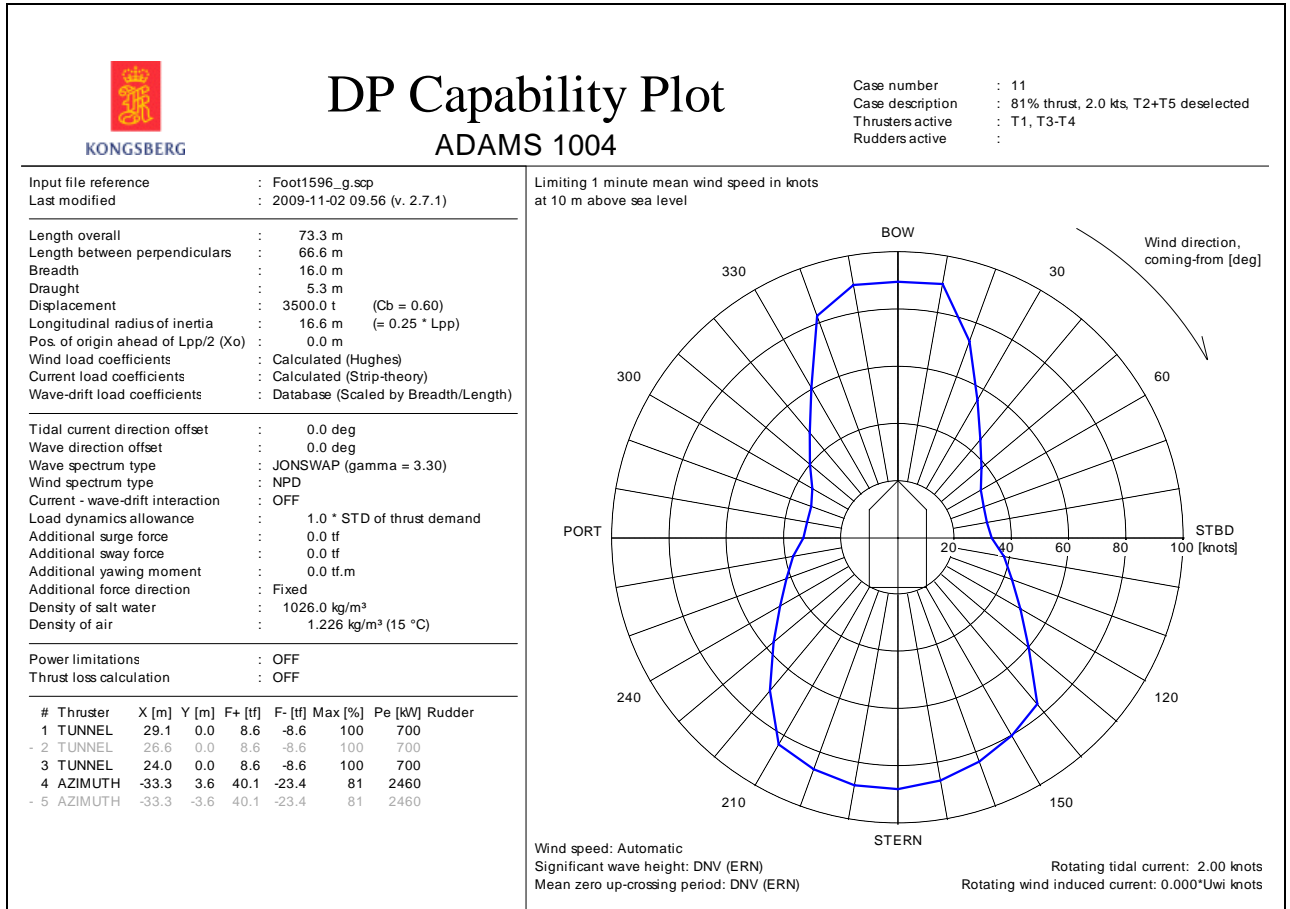
Figure 20: DP capability envelope for case 11.
