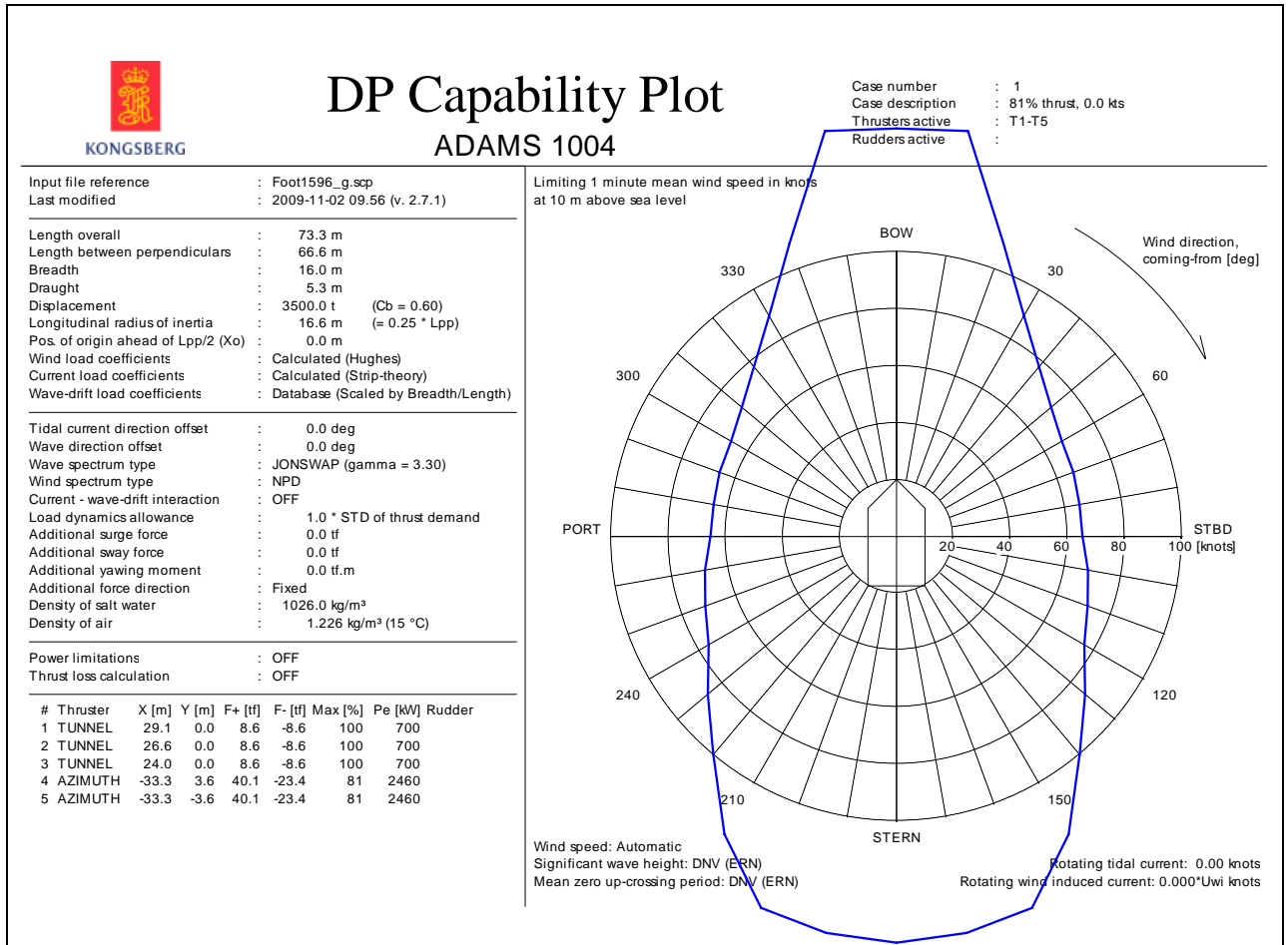
Figure 10: DP capability envelope for case 1.
