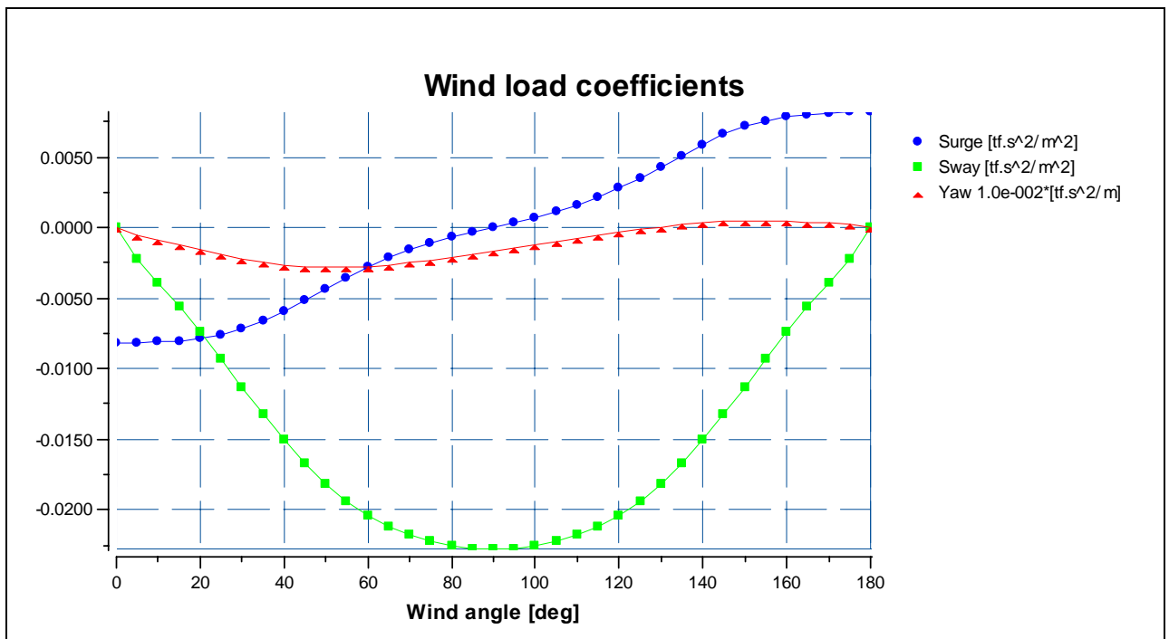
Figure 4: Wind load coefficients.
