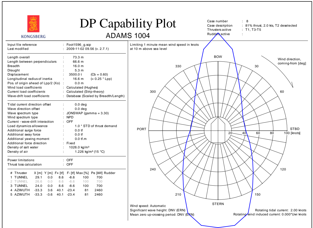
Figure 17: DP capability envelope for case 8.
