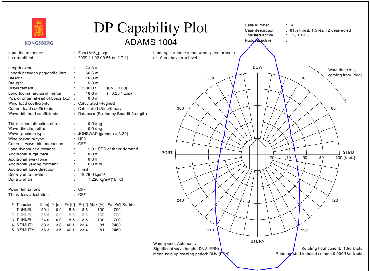
Figure 13: DP capability envelope for case 4.
