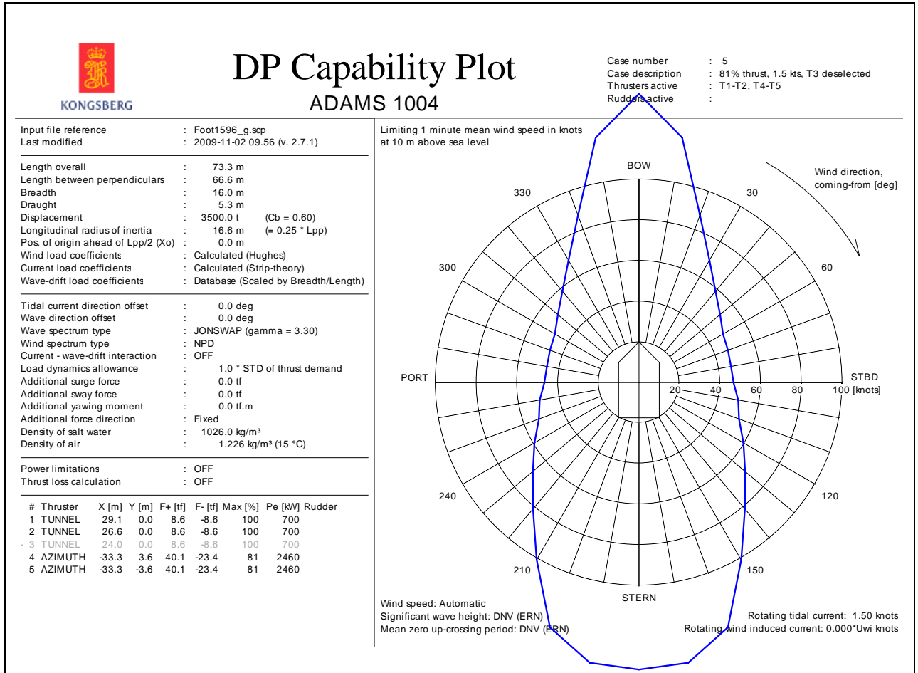
Figure 14: DP capability envelope for case 5.
