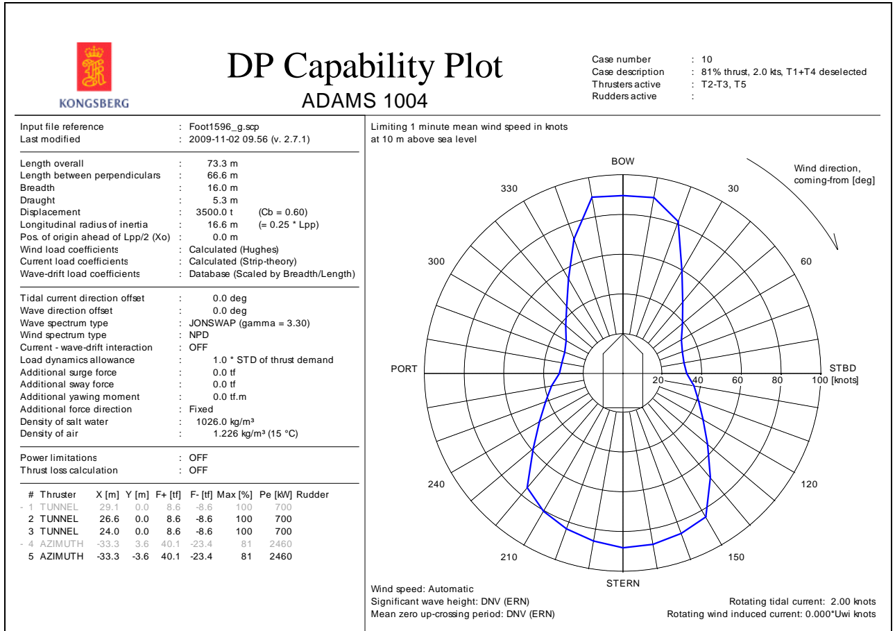
Figure 19: DP capability envelope for case 10.
