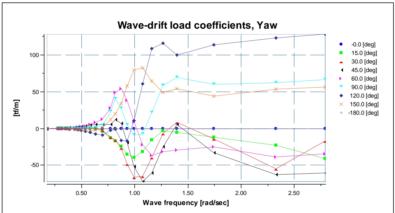
Figure 8: Wave-drift load coefficients for yaw.
