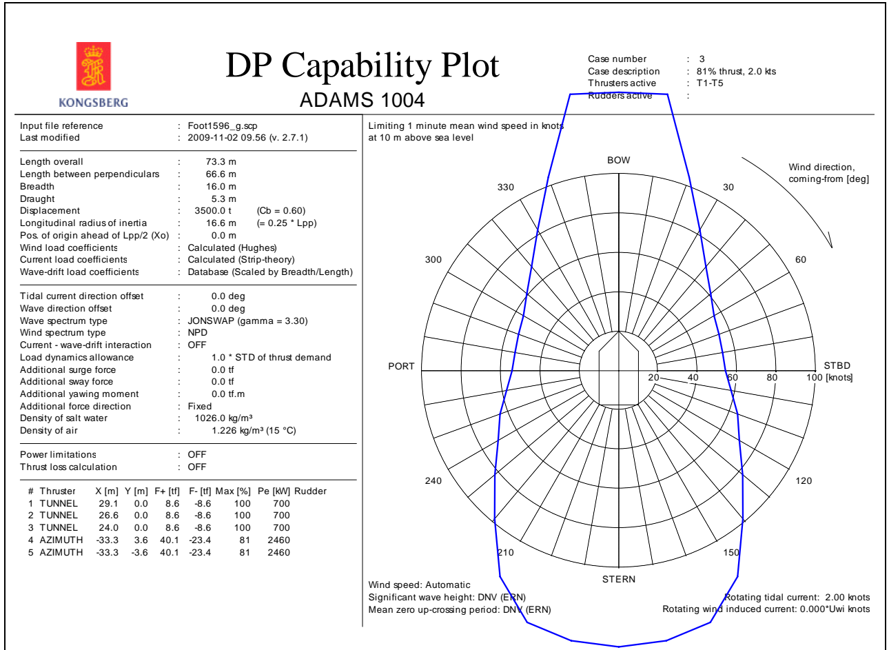
Figure 12: DP capability envelope for case 3.
