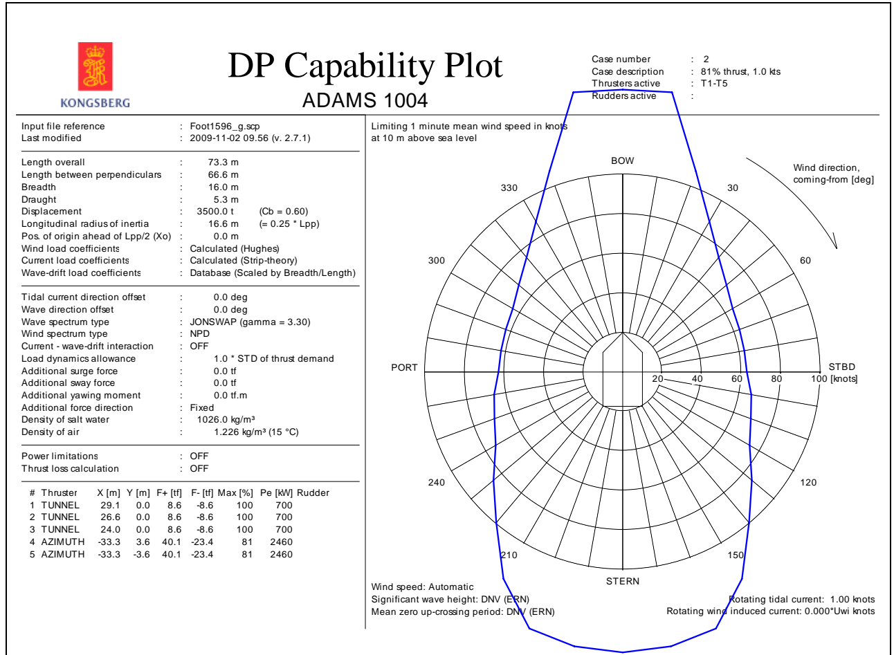
Figure 11: DP capability envelope for case 2.
