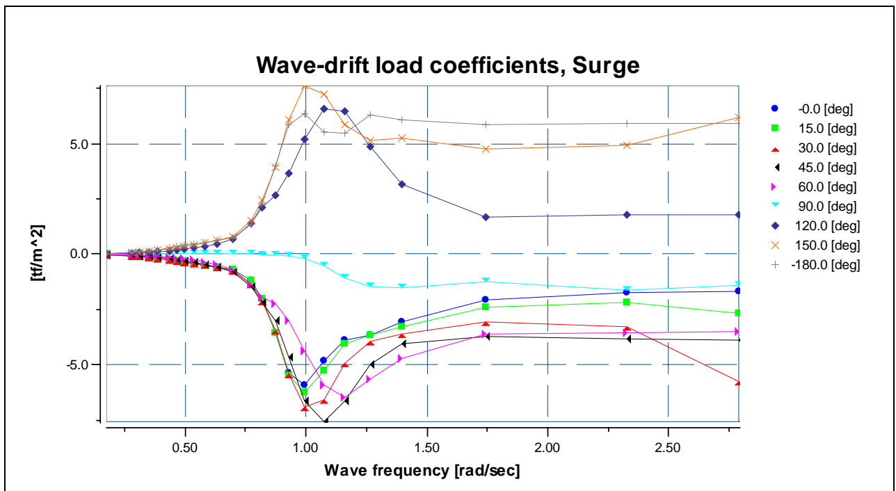
Figure 6: Wave-drift load coefficients for surge.
