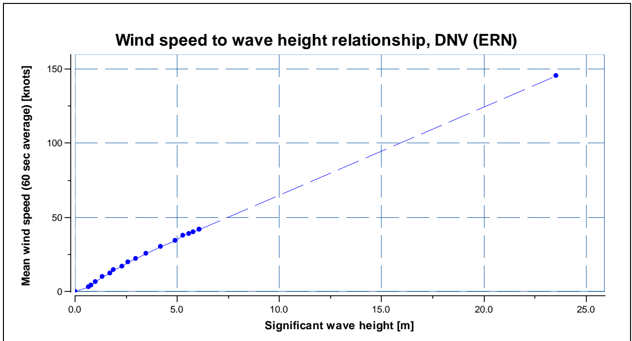
Figure 9: Wind speed to wave height relationship.
