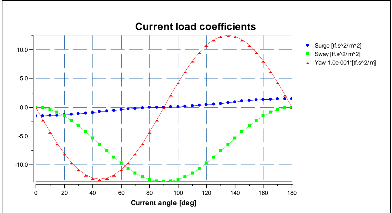
Figure 5: Current load coefficients.
