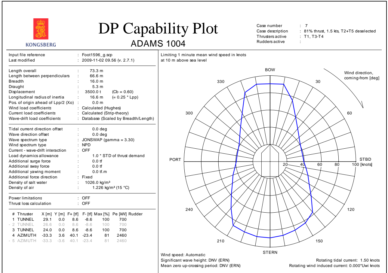
Figure 16: DP capability envelope for case 7.
