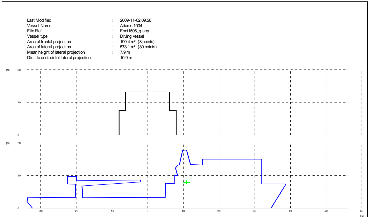
Figure 3: Wind area projections.
