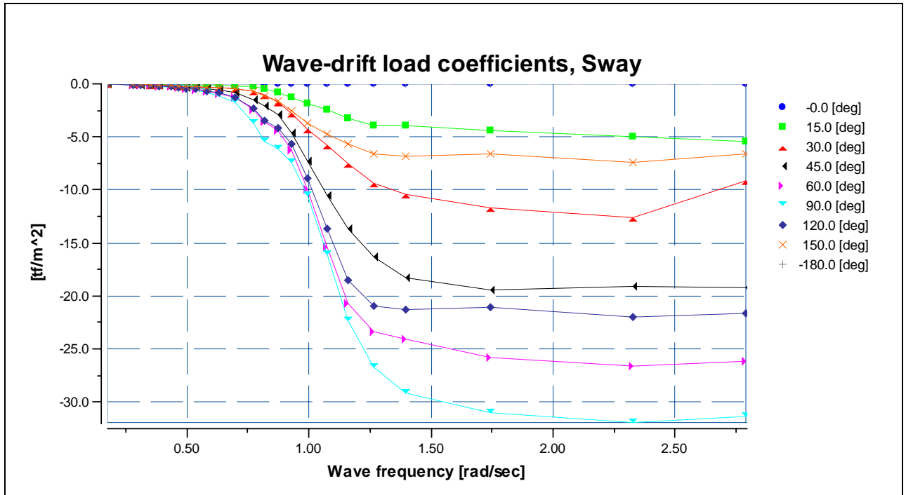
Figure 7: Wave-drift load coefficients for sway.
