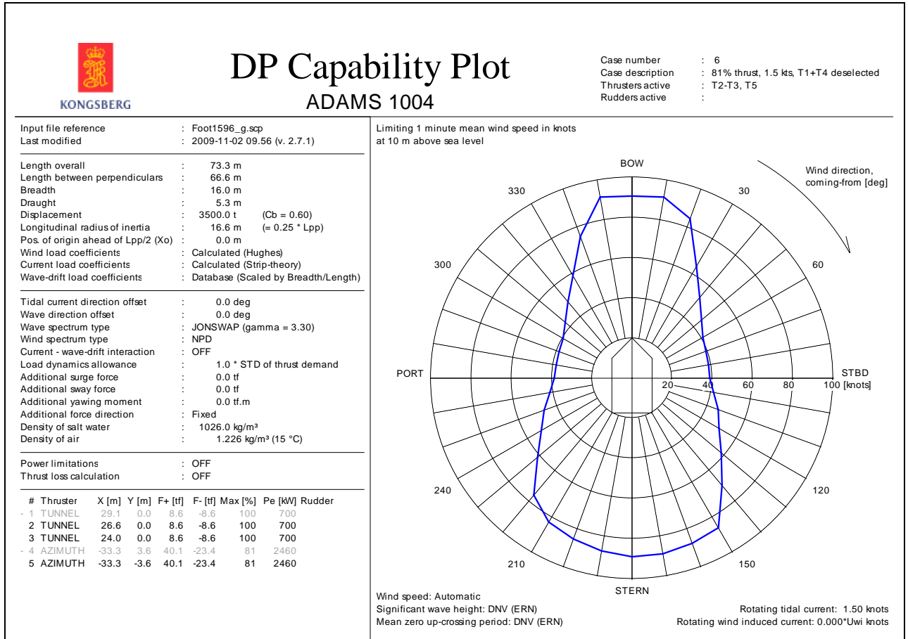
Figure 15: DP capability envelope for case 6.
